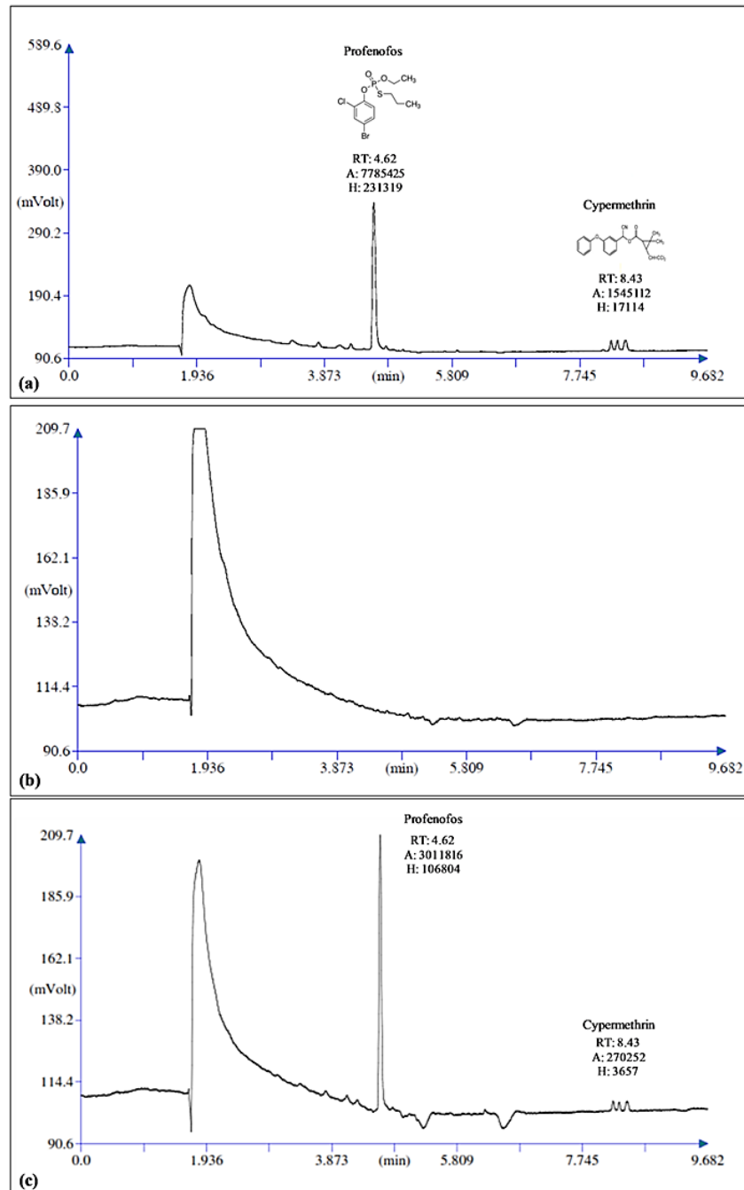
Figure 3. GC-chromatogram of profenofos and cypermethrin on GC-ECD (a) at standard 0.05 mg/kg (b) in control and (c) in sapota fruit sample at standard dose (SD)
